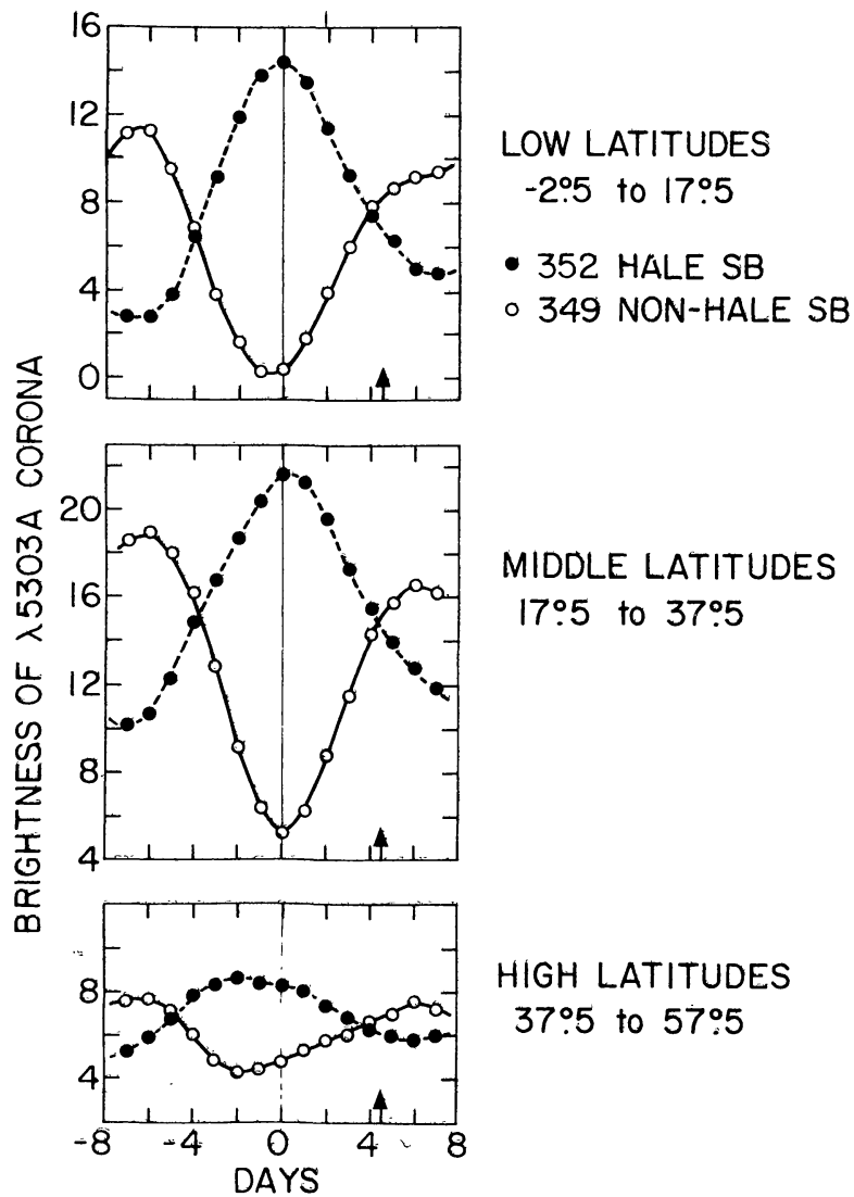
Fig. 3. Separate analysis for low ( -2.5^\circ to 17.5^\circ ), middle ( 17.5^\circ to 37.5^\circ ) and high ( 37.5^\circ to 57.5^\circ ) solar latitudes of the brightness of the green corona above Hale boundaries (filled circles) and above non-Hale boundaries (open circles). The coronal brightness is a maximum above Hale boundaries and a minimum above non-Hale boundaries in all three latitude ranges.
