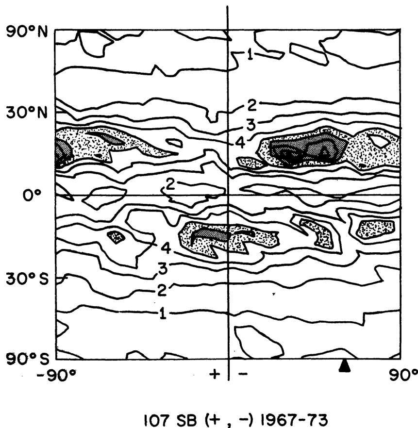
Fig. 6. Same as Figure 5, except for 107 (+, -) sector boundaries.
