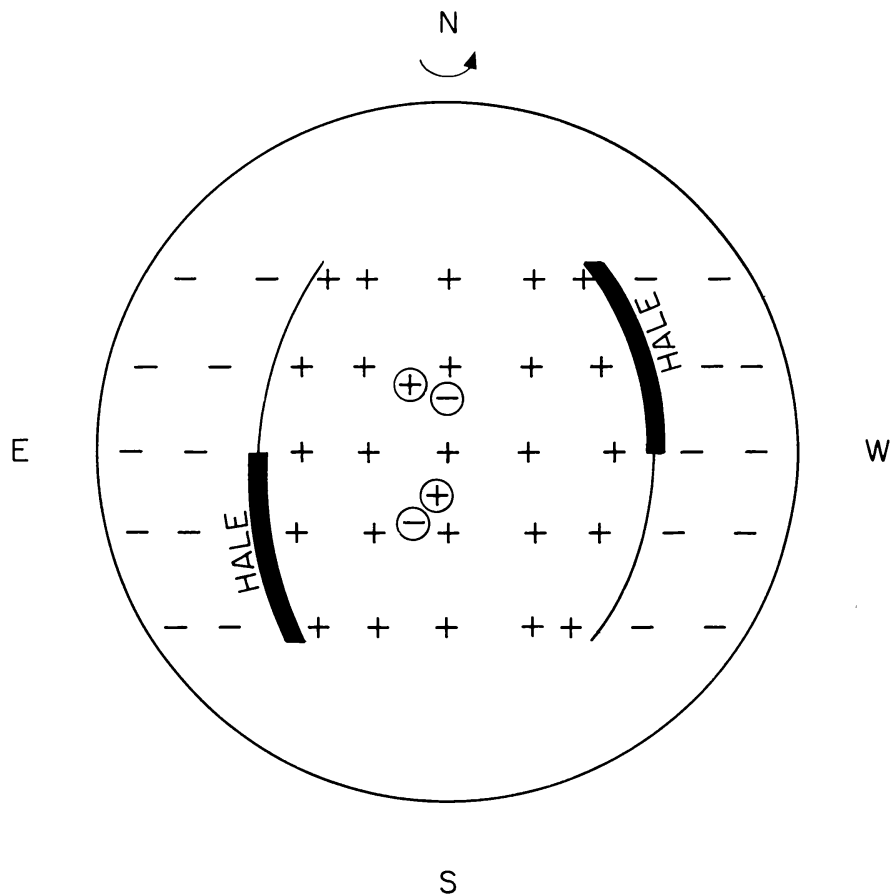
Fig. 1. Schematic of the solar disk showing the portion of a sector boundary that is designated a Hale boundary. A Hale boundary is that portion of a sector boundary that is located in the solar hemisphere in which the change of magnetic polarity at the sector boundary is the same as the change of magnetic polarity from a preceding spot to a following spot. The spot polarities shown in the small circles correspond to cycles 18 and 20.
