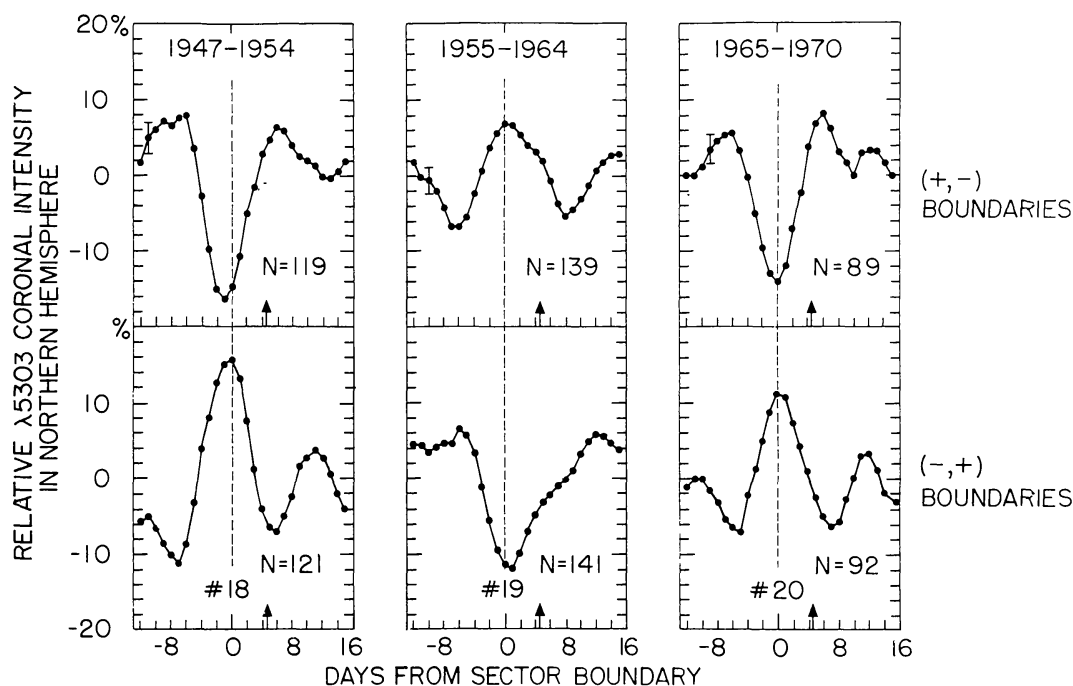
Fig. 2. Relative brightness in the northern hemisphere of the green coronal intensity on the Pic du Midi scale in sunspot cycles 18, 19 and 20 near (+, -) boundaries and near (-, +) boundaries. The vertical arrow indicates the time a sector boundary was observed at Earth, and the vertical dashed line indicates the location of the boundary on the Sun.
