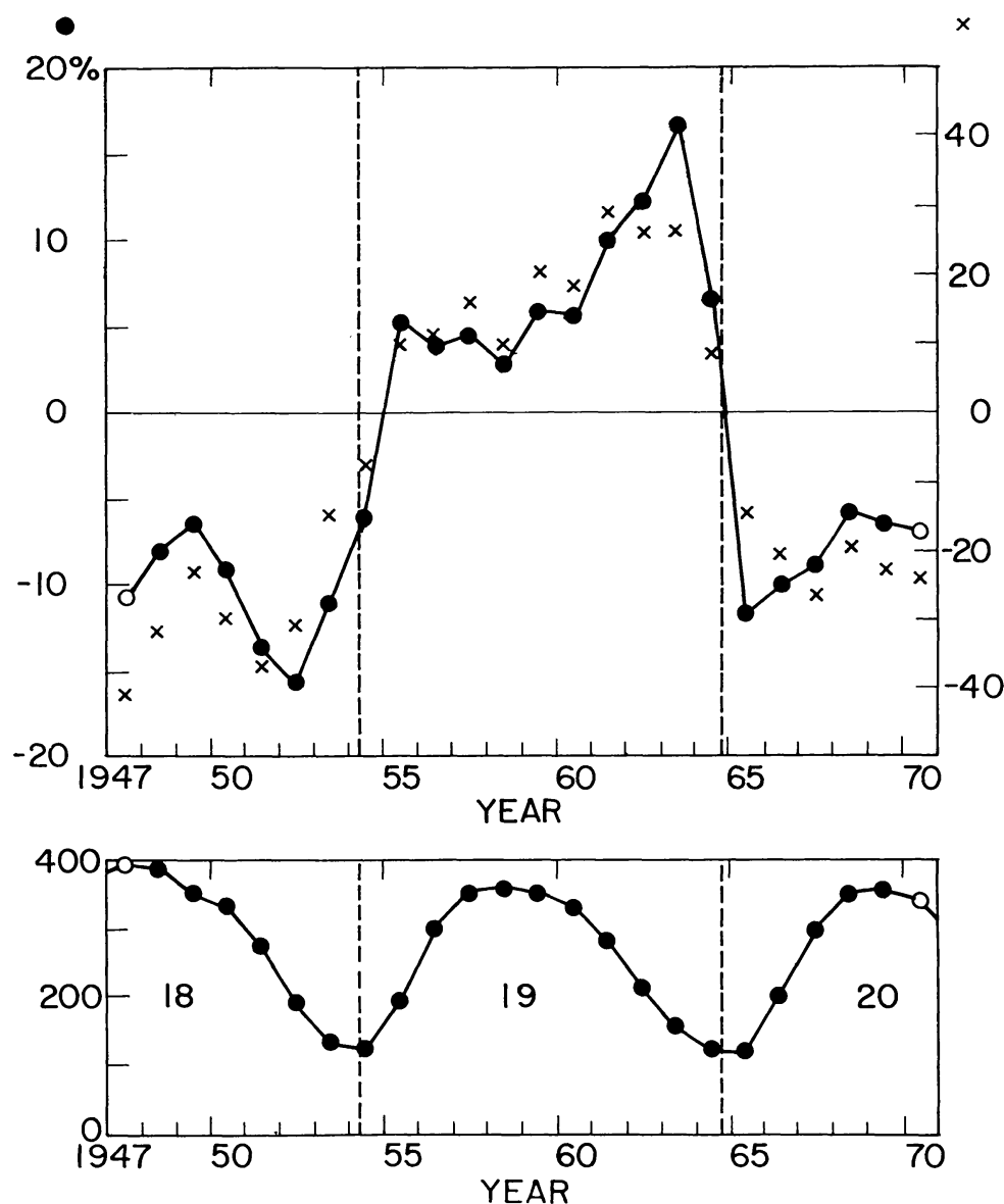
Fig. 4. Top : Relative coronal brightness above a (+,-) boundary in the northern hemisphere as a function of time from 1947 to 1970. During cycle number 19 (1954–1964) this portion of the boundary was a Hale boundary and had maximum coronal brightness, while at other times it was a non-Hale boundary and had minimum coronal brightness. The change from Hale boundary to non-Hale boundary is seen to occur within a year near the time of sunspot minimum. The left scale shows brightness changes in per cent, and the right scale in density units. Bottom : Total brightness of the green corona as a function of time from 1947 to 1970. The units are arbitrary.
